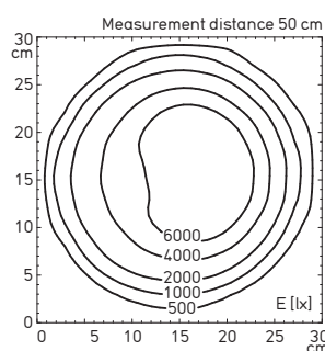
Illuminance with 24° angle of illumination (order no: 112 378 001)
