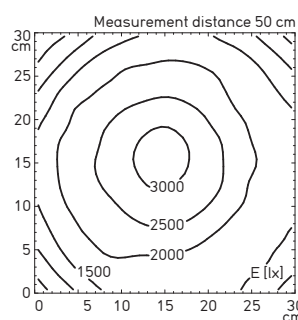
Illuminance with 36° angle of illumination (order no: 112 378 002)
