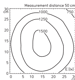
Illuminance with 60° angle of illumination (order no: 112 378 003)
