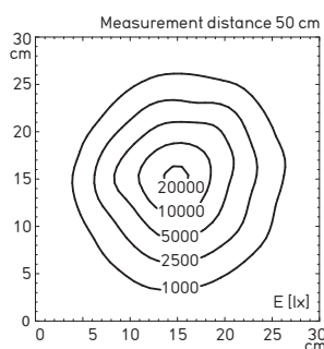
Illuminance with 10° angle of illumination (order no: 112 378 000)
